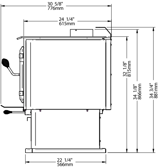
Figure 3: Side View
