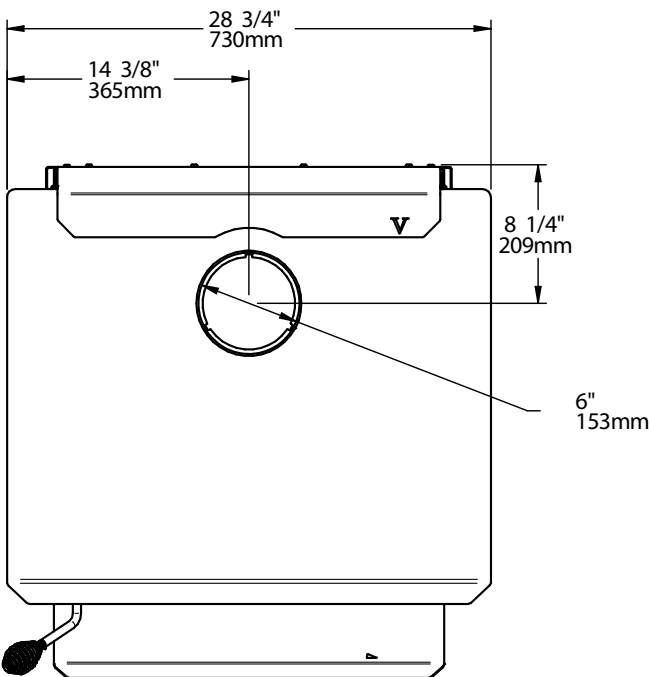
Figure 1: Top View
