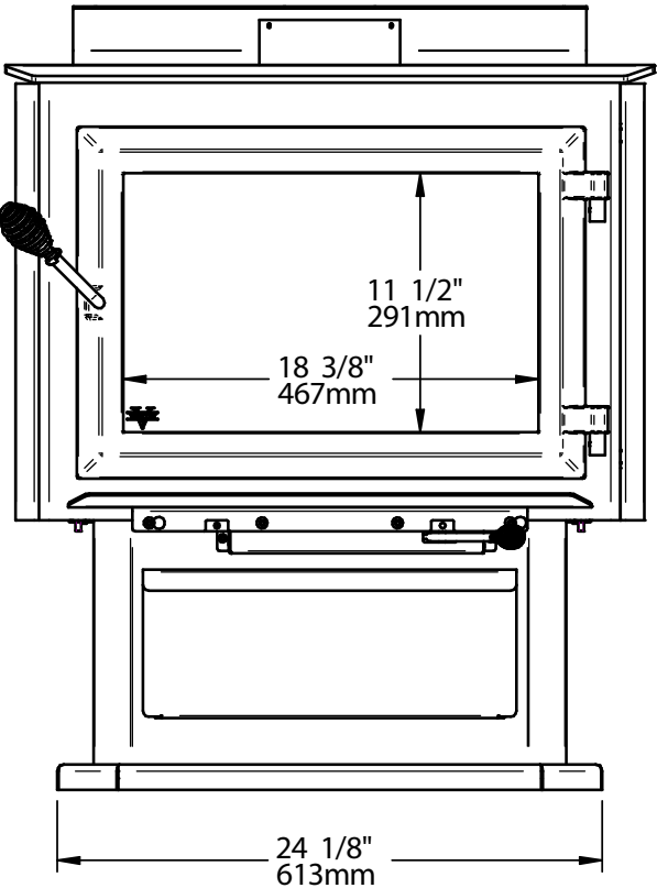
Figure 2: Front View
