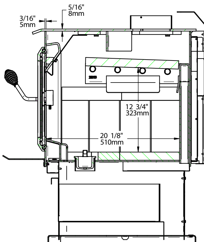
Figure 6: Side View - Combustion Chamber
