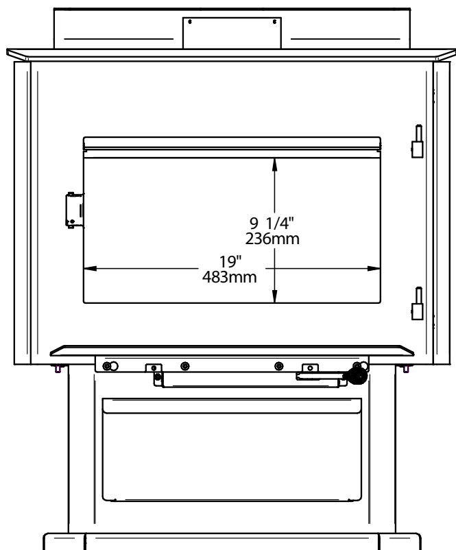
Figure 4: Door Opening
