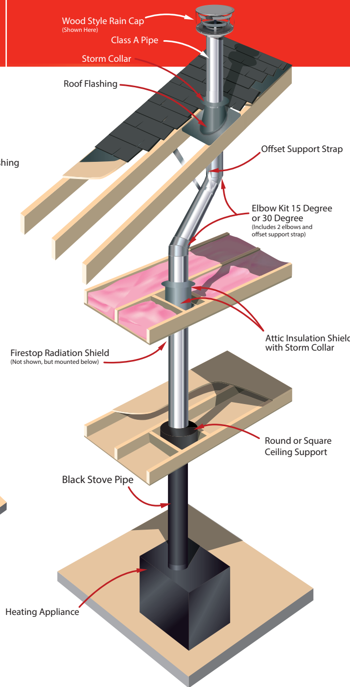
Offset Ceiling Support Installation
