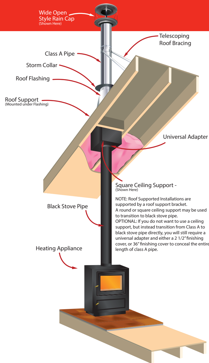
Roof Supported Installation
