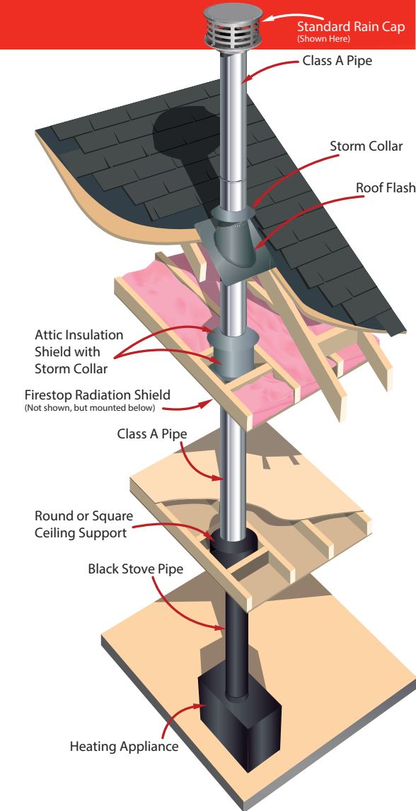
Ceiling Supported Installation
