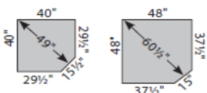
Single Cut Corner Dimensions
